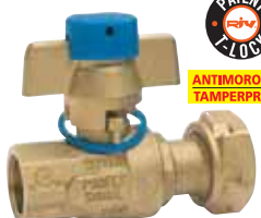
RIV 5130 - F/F 1/2" x 3/4" ▶ 3/4" x 1"
