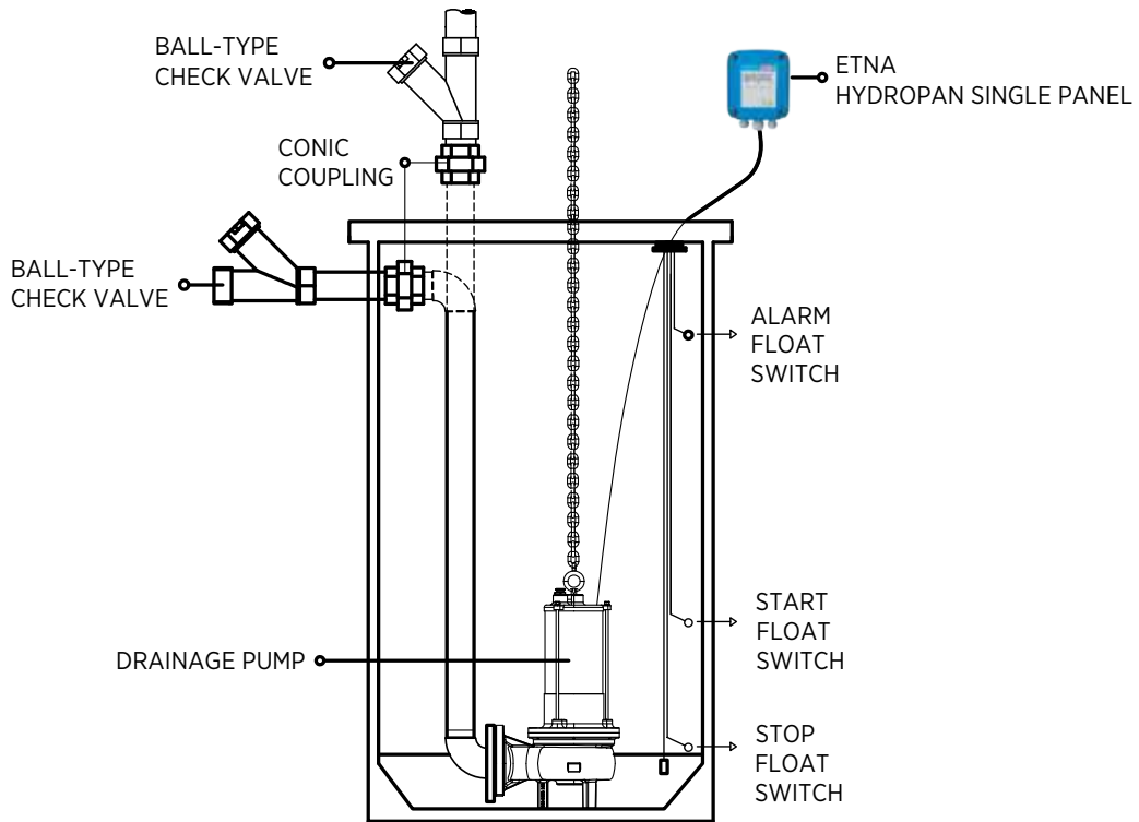
Fixed Installation (Pump can be detached from the conic coupling for easy maintenance)
