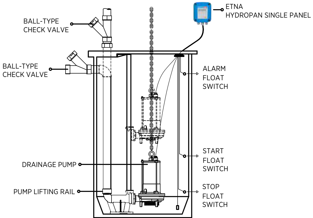
Fixed Installation with Lifting Rail (Pump can be removed for easy maintenance and repair)
